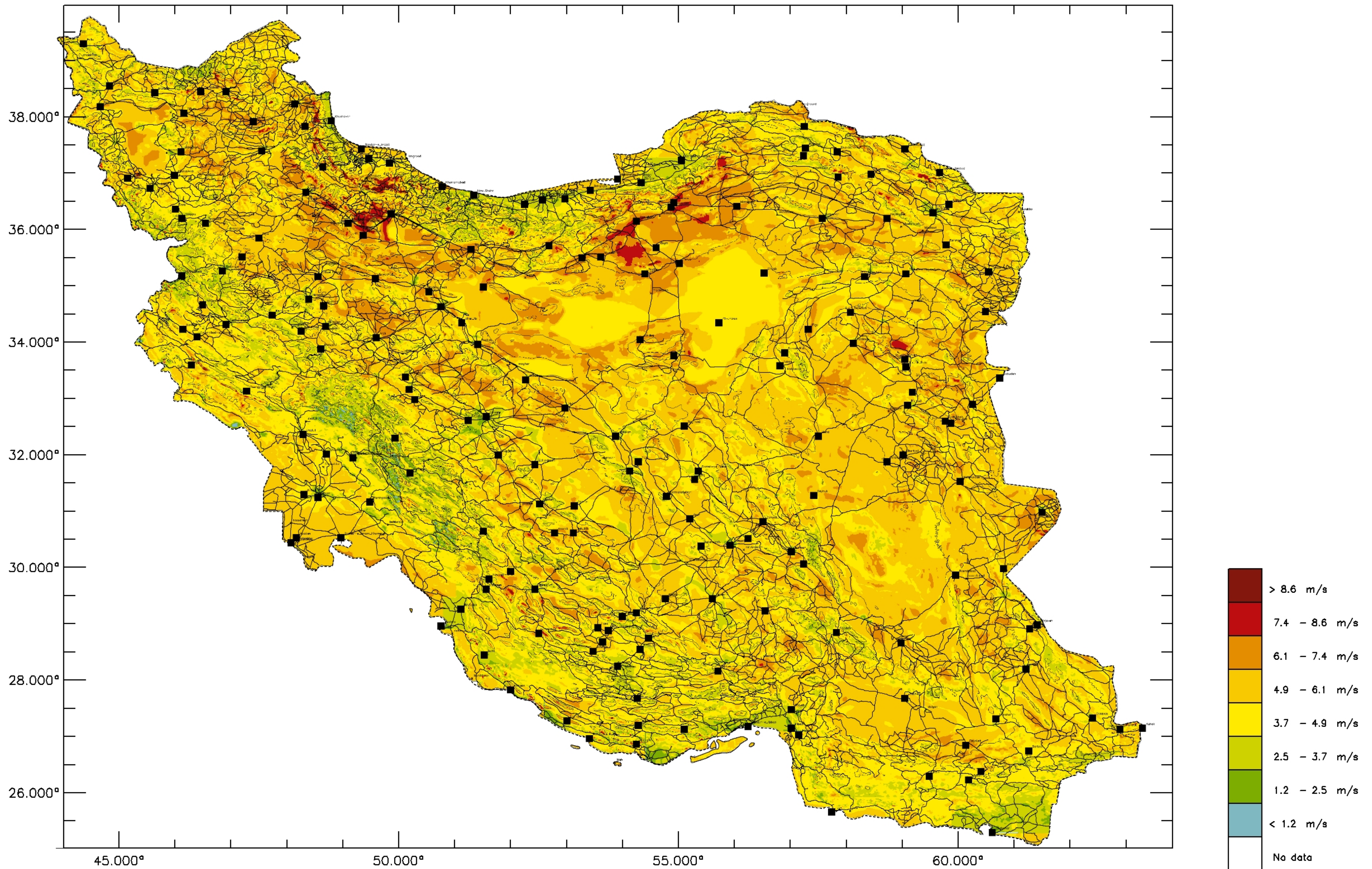
Mean Wind Velocity at Height 40 m a.g.l.
