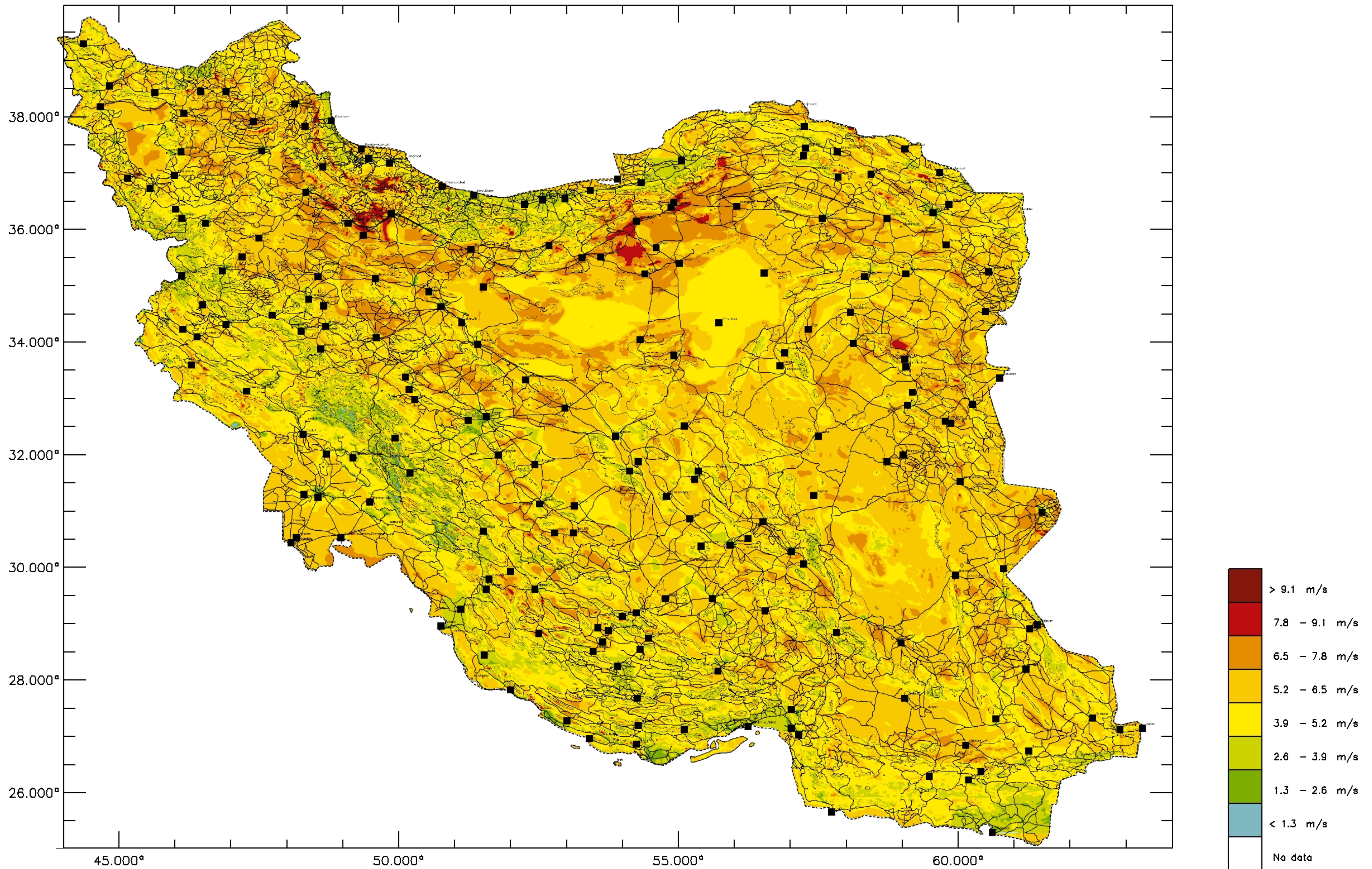
Mean Wind Velocity at Height 60 m a.g.l.
